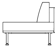
30004 Single module W 83,0 cm / 32.7" D 90,0 cm / 35.4" H 64,5 cm / 25.4" SH 39,5 cm / 15.6" Net/Gross weight 17,4 kg / 26,2 kg Volume 0,56 m 3 Unit 1 pc
