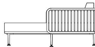
30011 Daybed L 163,0 cm / 64" D 160,0 cm / 63" H 64,5 cm / 25.4" SH 39,5 cm / 15.6" Net/Gross weight 51,6 kg / 74,2 kg Volume 1,85 m 3 Unit 1 pc
