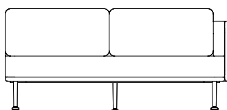
30008 Daybed module left L 160,0 cm / 63" D 160,0 cm / 63" H 64,5 cm / 25.4" SH 39,5 cm / 15.6" Net/Gross weight 47,5 kg / 72,6 kg Volume 1,82m 3 Unit 1 pc
