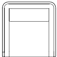
30004 Single module W 83,0 cm / 32.7" D 90,0 cm / 35.4" H 64,5 cm / 25.4" SH 39,5 cm / 15.6" Net/Gross weight 17,4 kg / 26,2 kg Volume 0,56 m 3 Unit 1 pc
